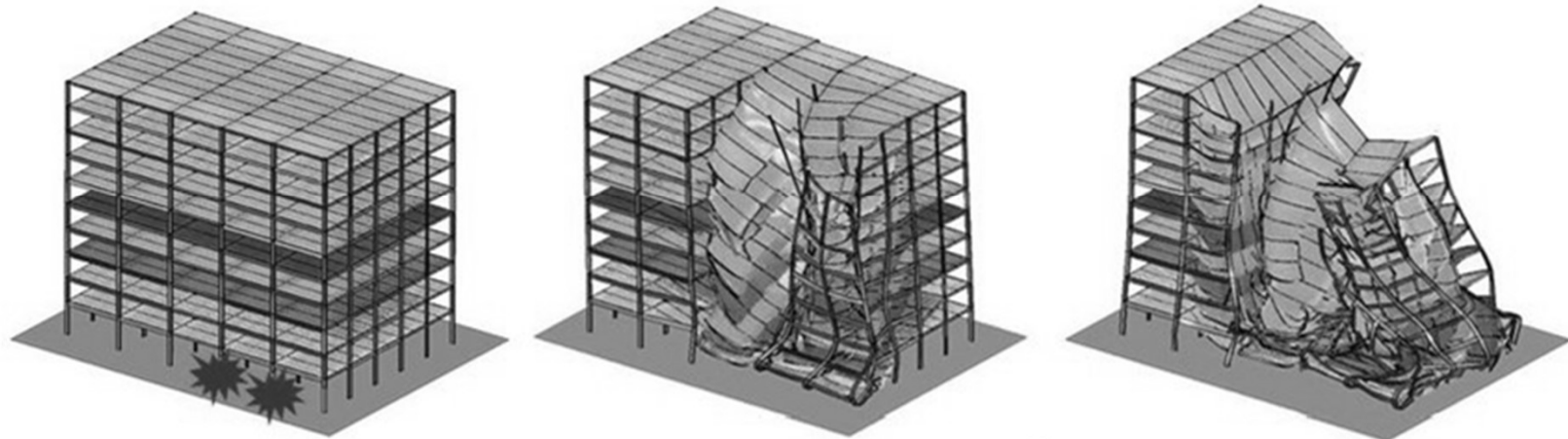
Progressive Collapse Mechanism (Failure of structural members one after another)
