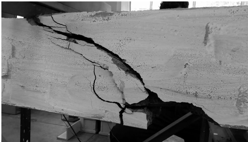
Rupture (Flexure, shear or combination )
