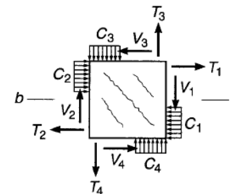
Lateral Load
